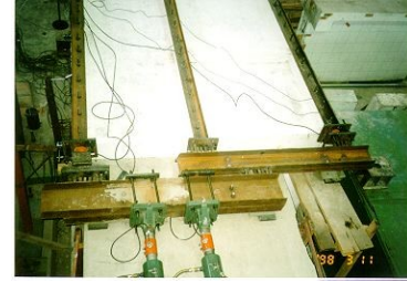
Photo 6. Specimen During Testing
